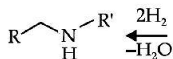
Scheme 1. General Sche C-O cleavage
